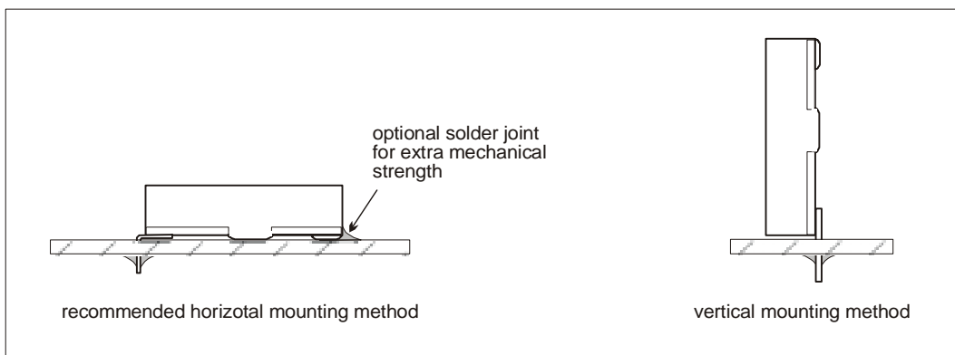
Figure 3: Module mounting options
