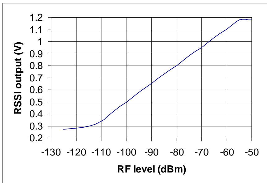
Figure 2: RSSI response curve
