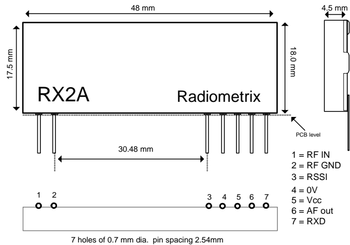
Figure 1: Physical dimensions
