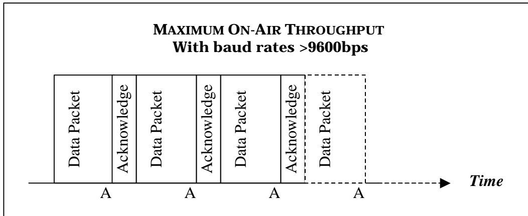
Figure 5: A SPACEPORT MODEM pair streaming at maximum throughput
