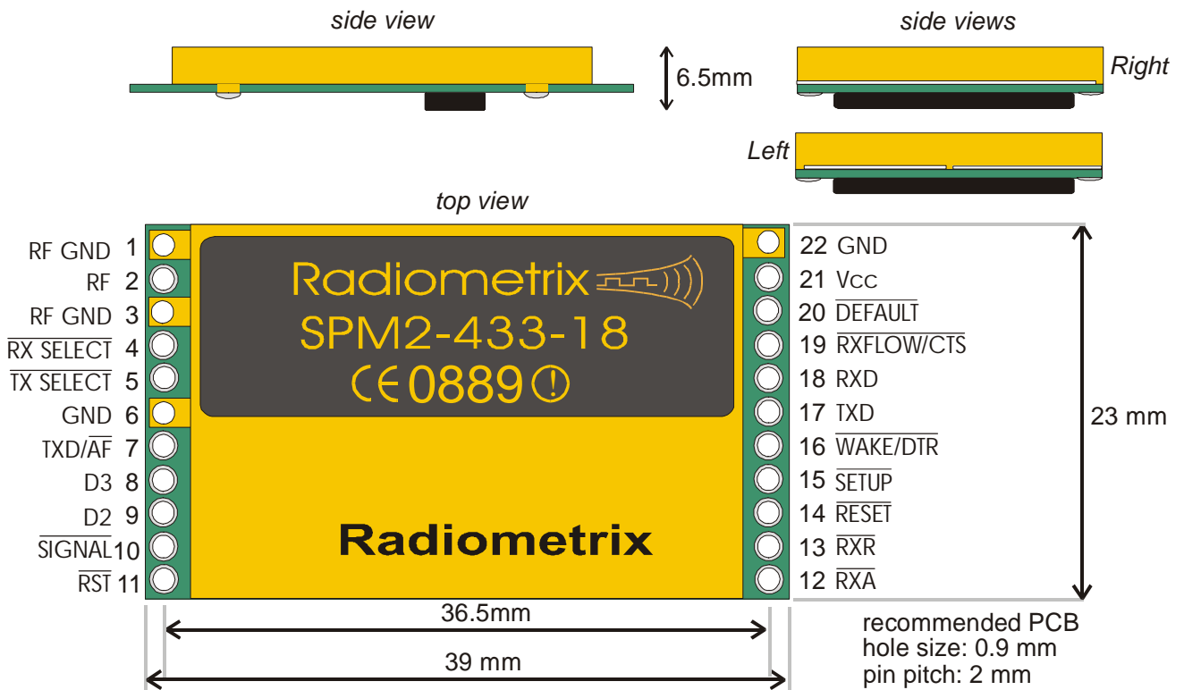
Figure 2: Physical dimensions and pinouts
