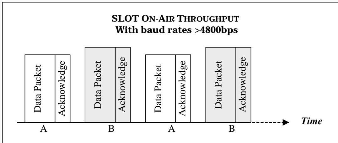
Figure 6: Two SpacePort Modem pairs operating Slot throughput
