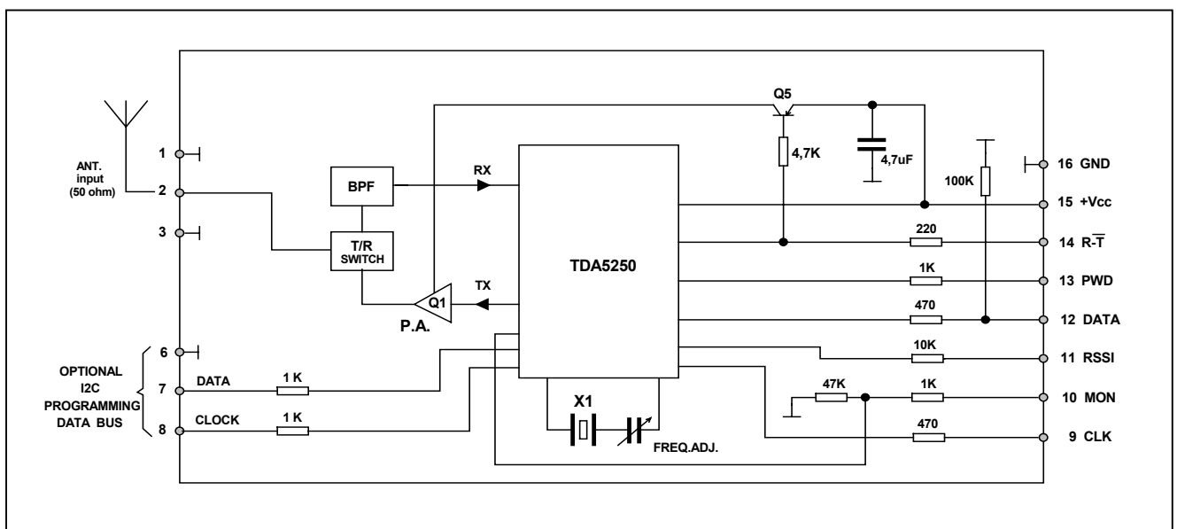
Block diagram
