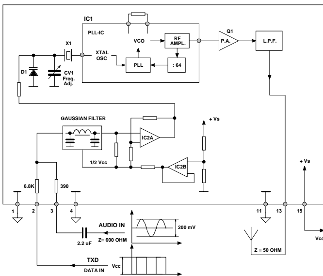
Fig.1 – BT37S – Block diagram.
