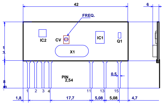
Fig.2 – BT37S – Physical dimensions.
